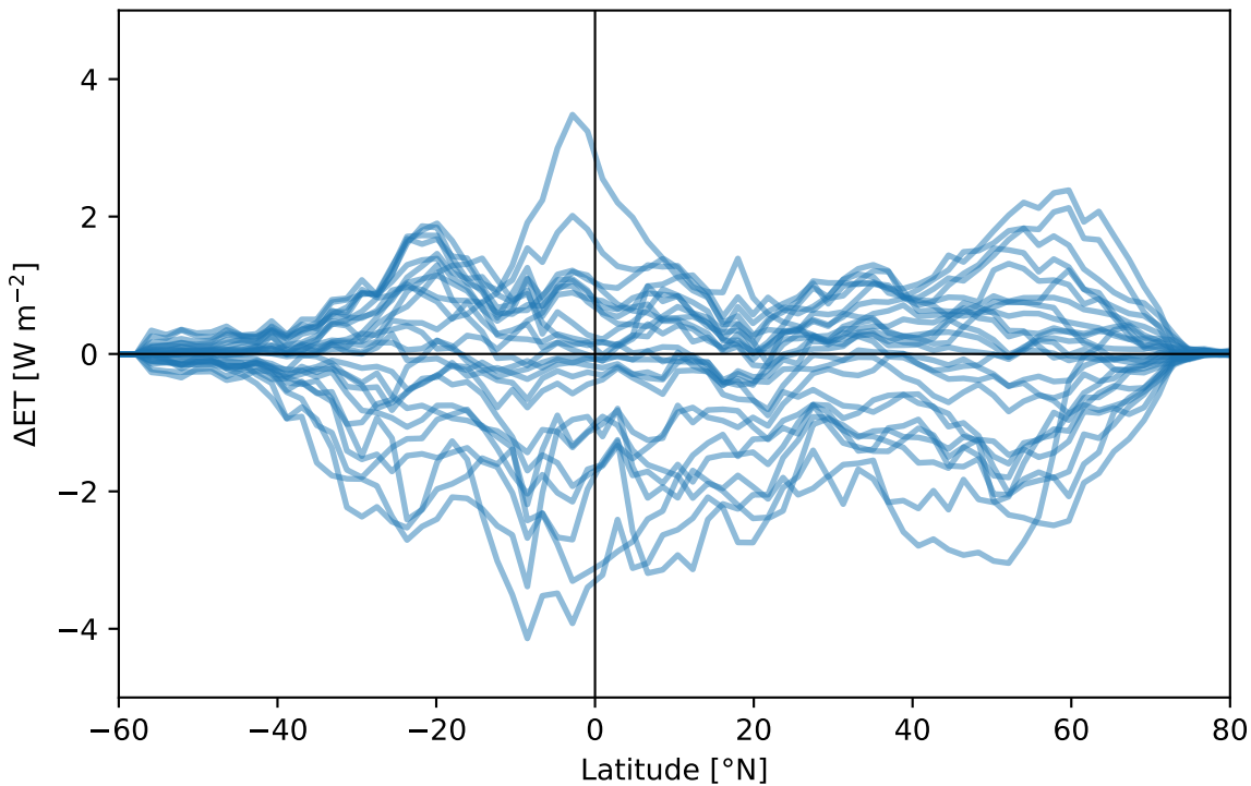
Zonal-mean \Delta ET across FHIST PPE; time mean 1995-2014
