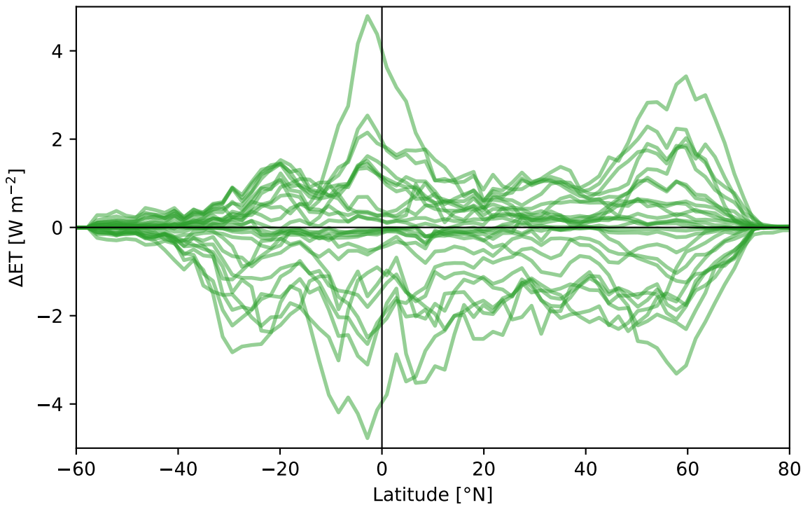
Zonal-mean \Delta\text{ET} across OFFLHIST PPE; time mean 1995-2014
