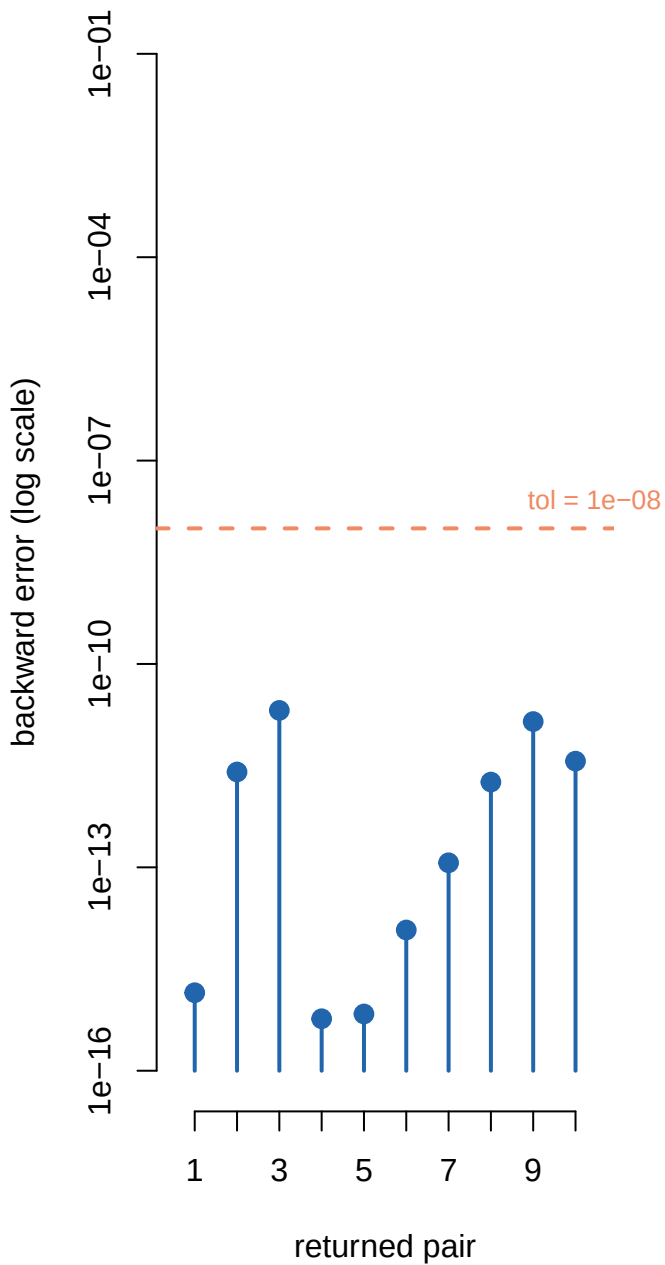
largest(): passed
