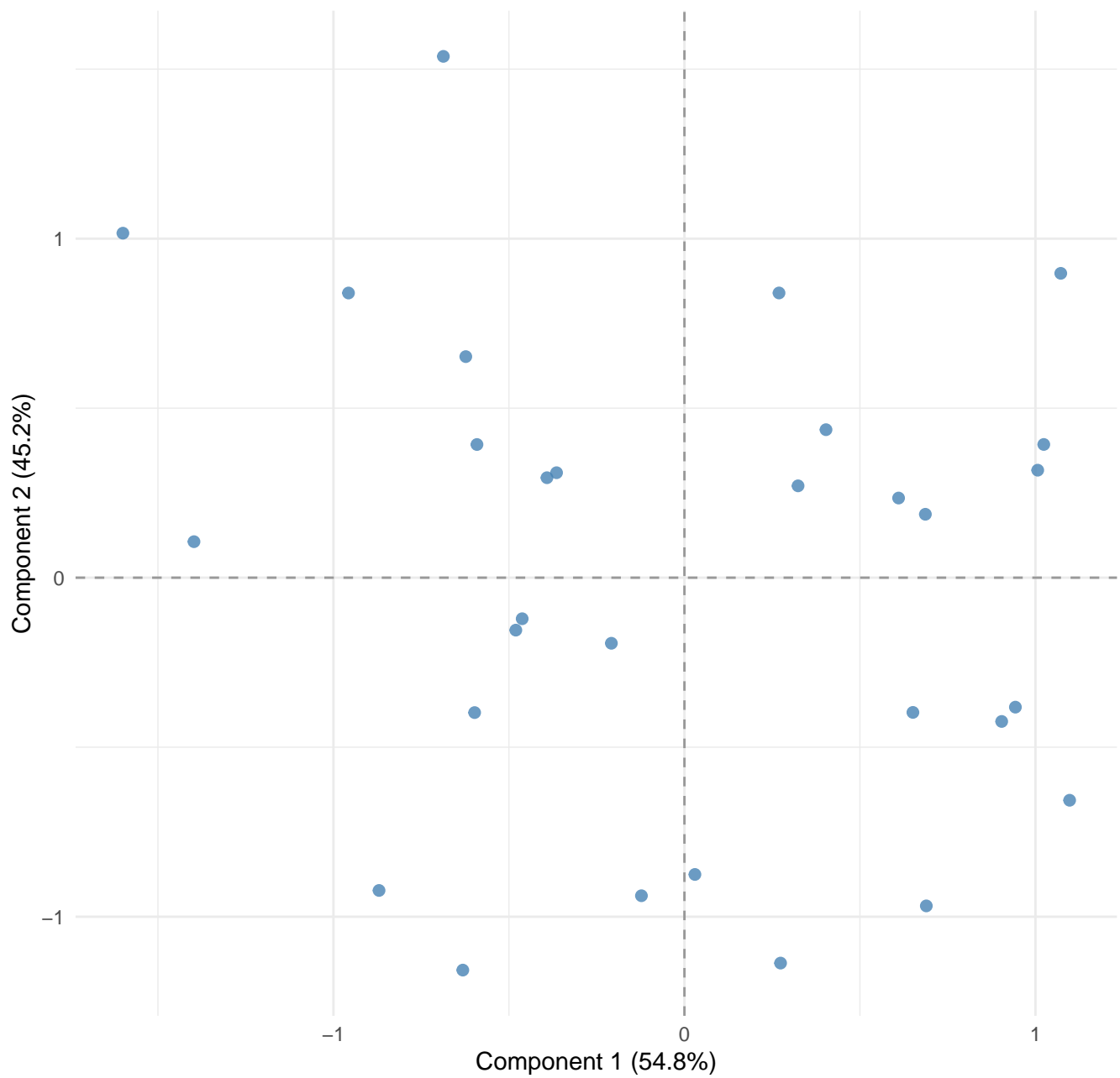
Penalized MFA Consensus Scores
