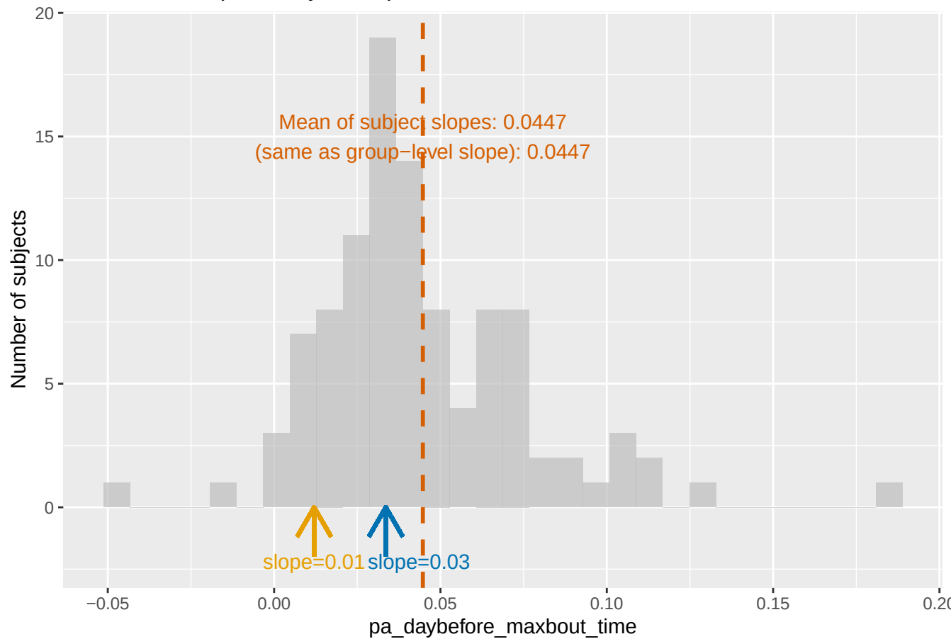
Distribution of per-subject slopes
