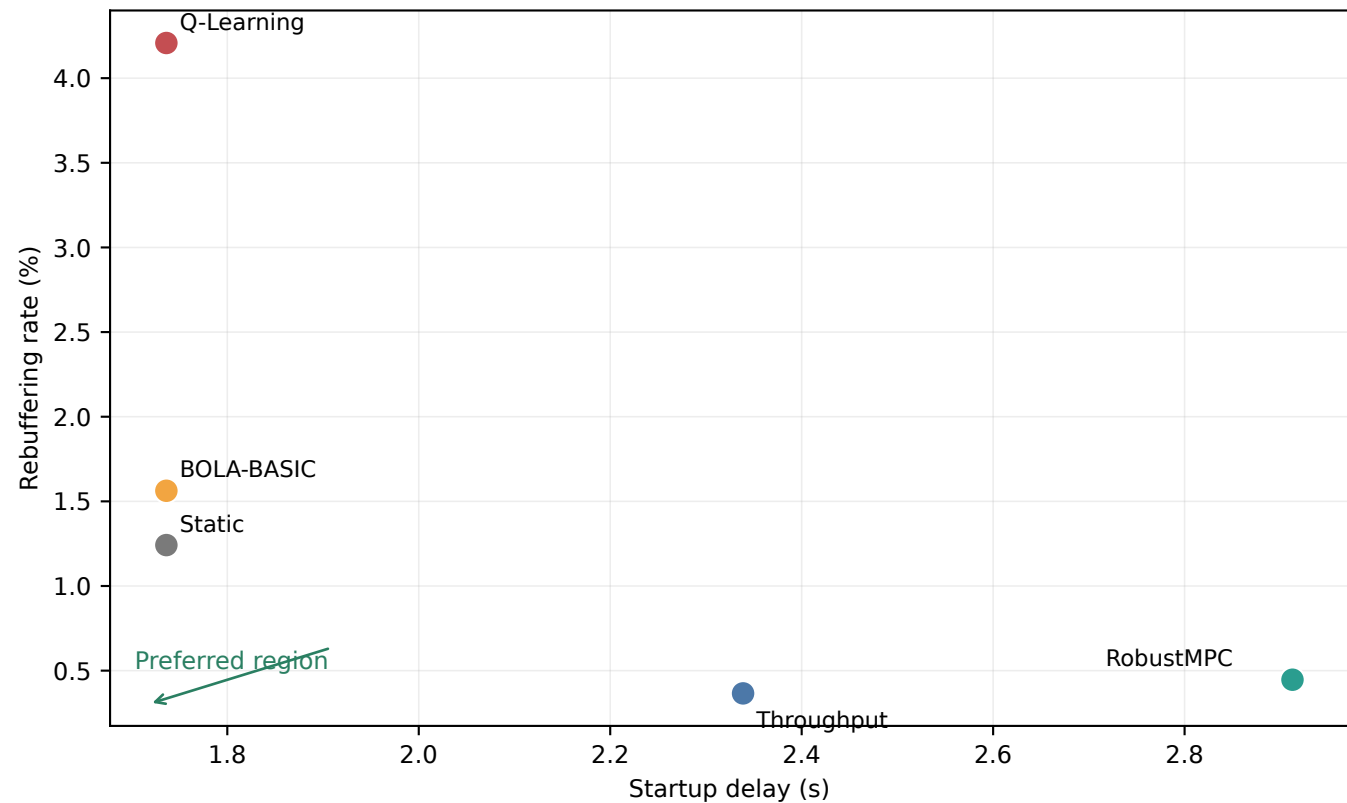
Startup-rebuffering trade-off
