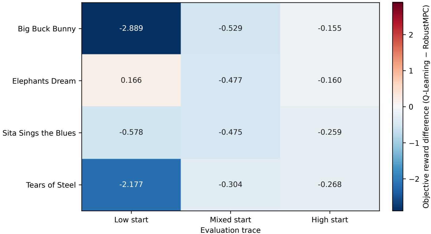
Primary contrast by content and evaluation trace
