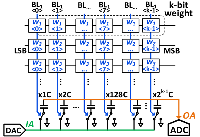
Fig. 7. Basic idea of a binary weighted capacitor ladder-based multibit multiplier for CiM.
