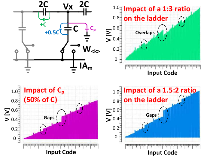
Fig. 11. Non-ideal 1:2 ratio and parasitic capacitance on the proposed C-2C capacitor ladder can cause gaps, overlaps, and dynamic range scaling on the TC.
