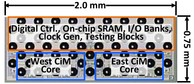
Fig. 20. Micrograph of the proposed analog CiM test chip.
