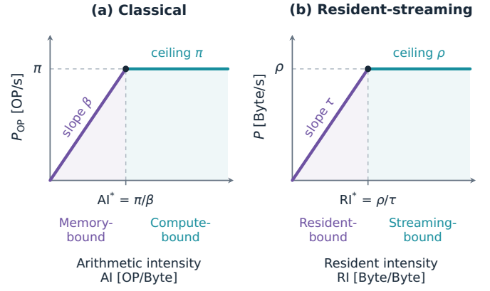
Fig. 2. Matched Roofline geometry with different service meanings: (a) compute capacity \pi and memory bandwidth \beta [1]; (b) streaming capacity \rho and resident-write capacity \tau . Linear-axis schematics use independent scales; the curves are upper bounds.
