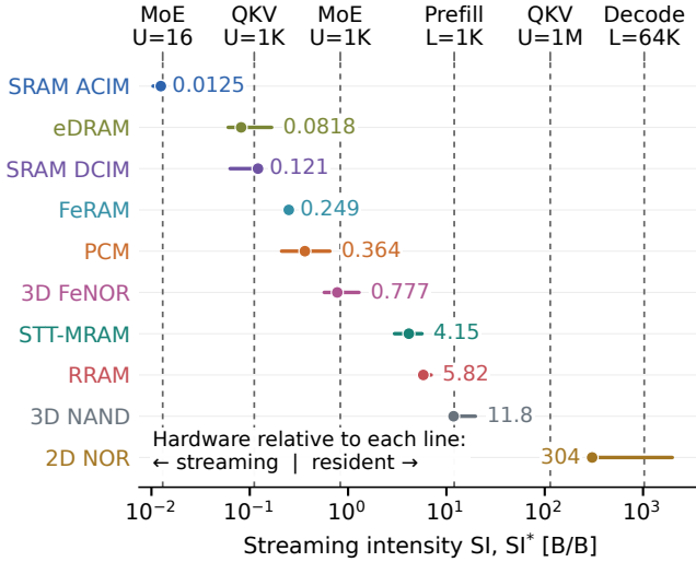
Fig. 4. Full-load critical reuse U^* = T_R/\Delta_S = N\text{SI}^* at equal byte widths; each row uses its native W[N, K] . Numbers give typical values; segments span only three paired scenarios. Dashed lines mark illustrative reuse counts, not universal balance points. 1K = 1024 .
