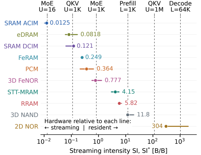
Fig. 4. Full-load critical reuse U^* = T_R/\Delta_S = N\text{SI}^* at equal byte widths; each row uses its native W[N, K] . Numbers give typical values; segments span only three paired scenarios. Dashed lines mark illustrative reuse counts, not universal balance points. 1K = 1024.
