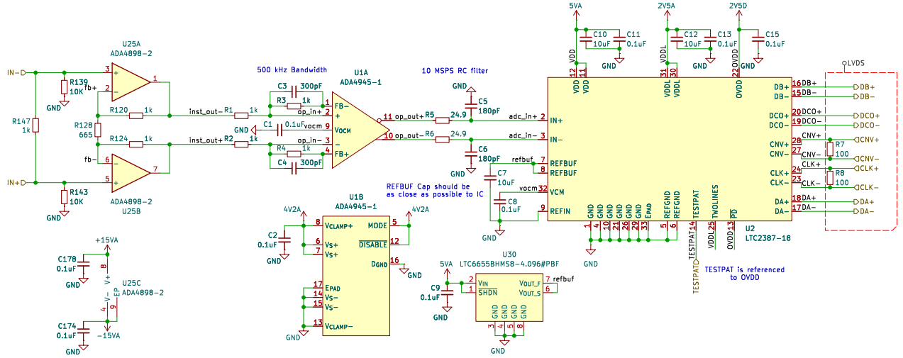
Figure 9: Analog Front-End and ADC Circuit.
