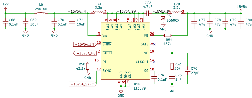
Figure 6: Analog -15.5 V Inverting DC-DC Converter Circuit
