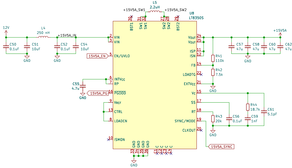
Figure 5: Analog 15.5 V Buck-Boost DC-DC Converter Circuit
