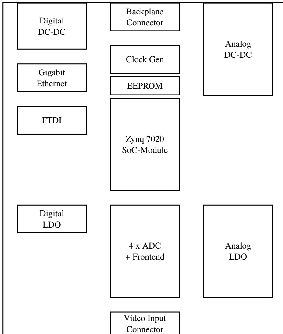
Figure 1: PCB Block-diagram of the 16.2 cm x 17.1 cm, six-layer PCB with impedance control, 4-channel ADC prototype board.
