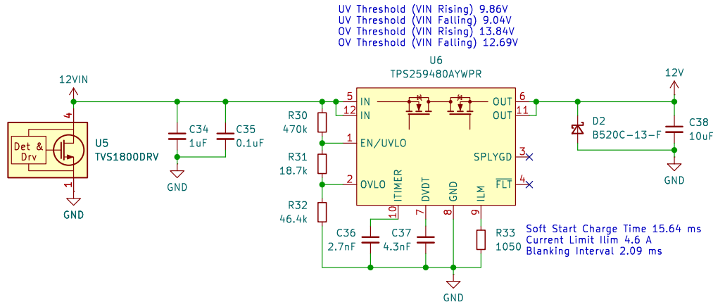
Figure 2: 12 V Input Protection Circuit
