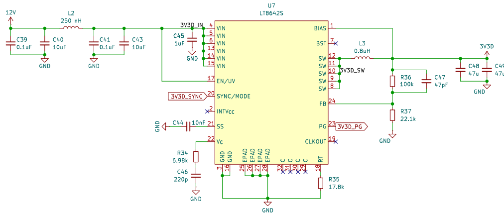
Figure 3: Digital 3.3 V Step-Down DC-DC Converter Circuit
