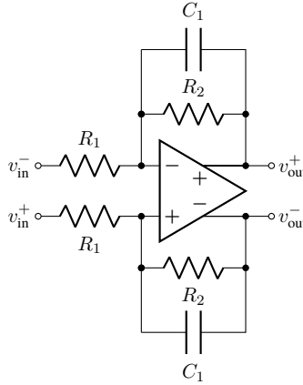
Figure 11: Fully Differential Amplifier Equivalent Circuit.
