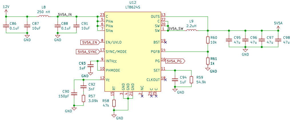
Figure 4: Analog 5.5 V Step-Down DC-DC Converter Circuit
