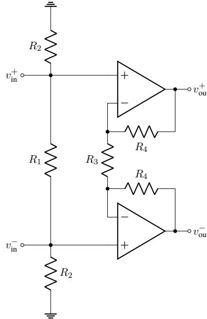
Figure 10: Instrumentation Amplifier Equivalent Circuit.
