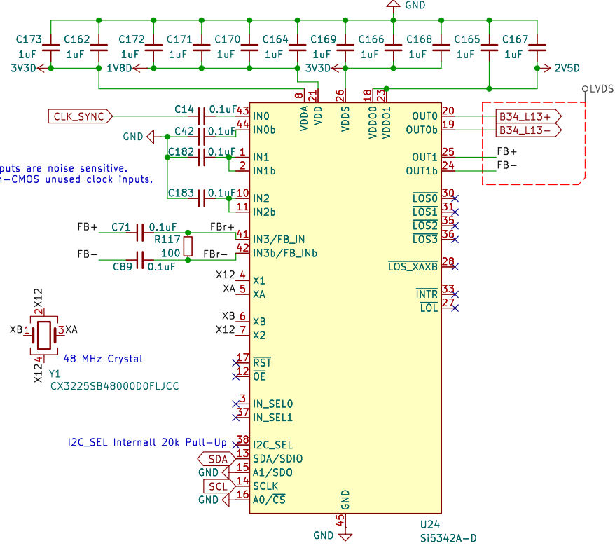
Figure 8: Si5342A-D Clock Generator Jitter Attenuator Circuit
