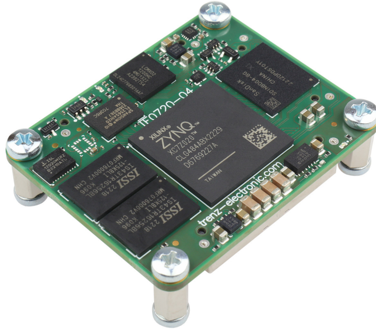
Figure 13: Trezz Electronic TE0720-04-62I33MA SoC-Module.
