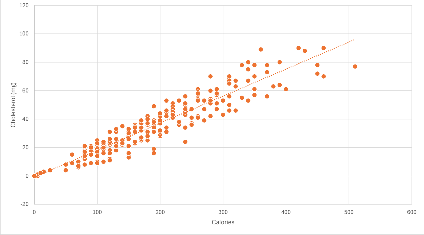
Field: Calories and Field: Cholesterol (mg) appear highly correlated.
