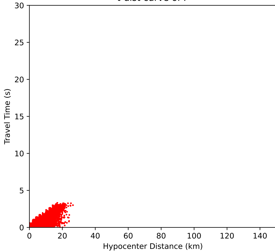
t-dist curve of P
