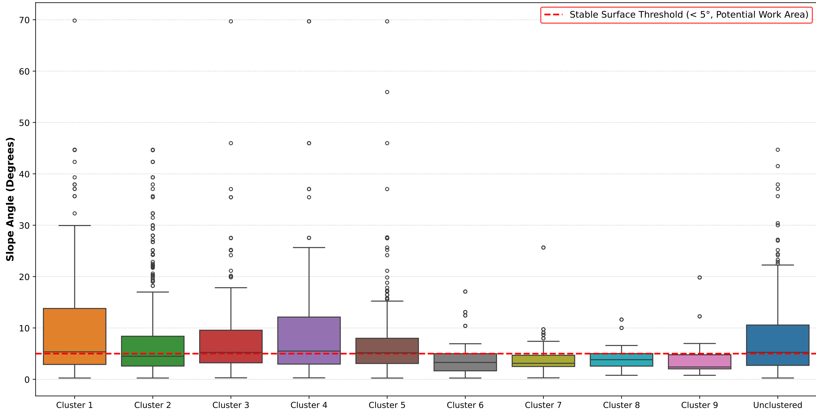
Surface Stability: Slope Gradient per Cluster (All 9 DBSCAN Clusters & Unclustered)
