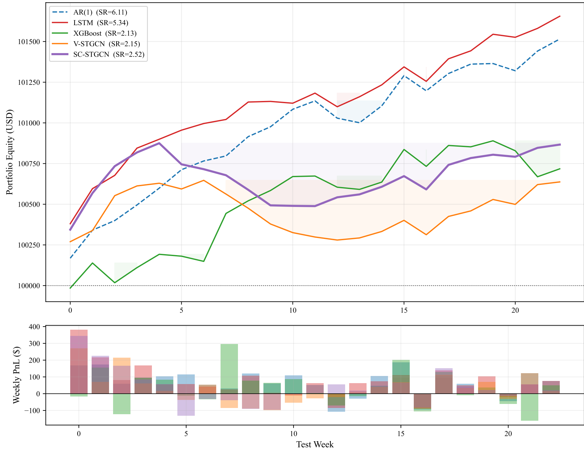
Long-Short CDS Protection Strategy — DELTA Forecasts
