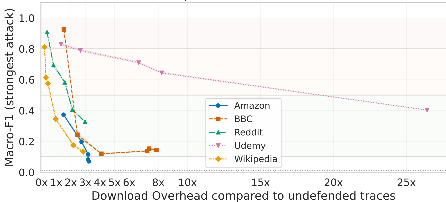
Calibration plot for the CL-Tamaraw defense
