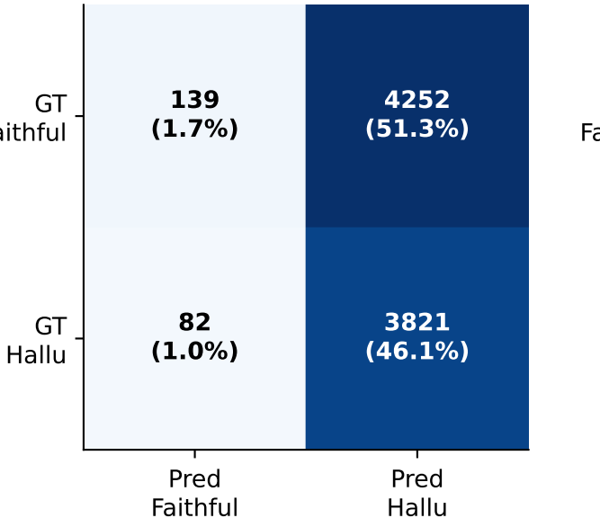
CheXagent-8B
