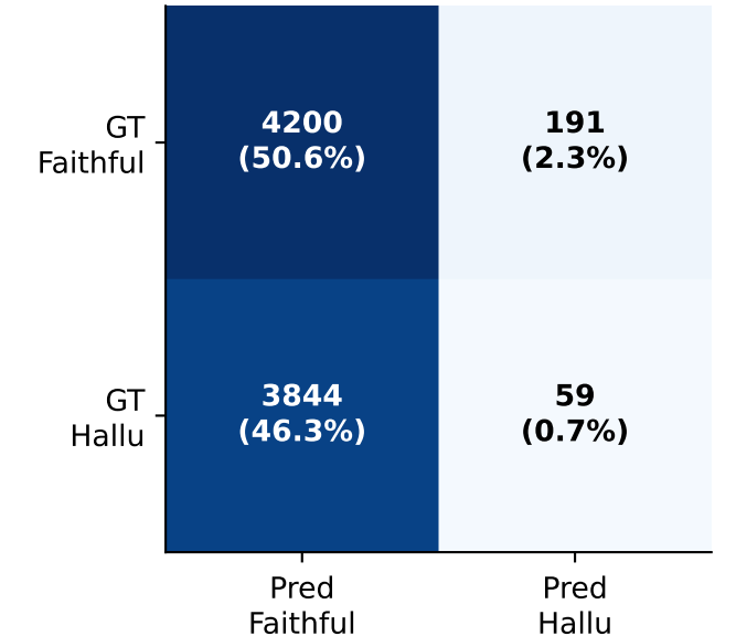
BiomedCLIP-300M
