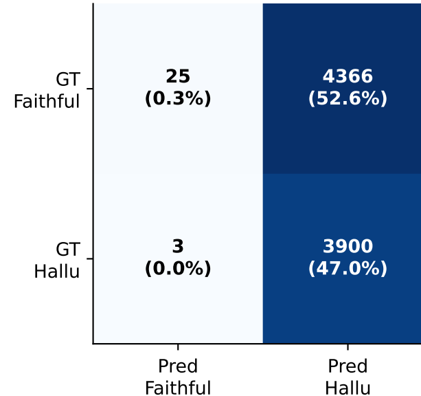
Qwen2.5-VL-7B
