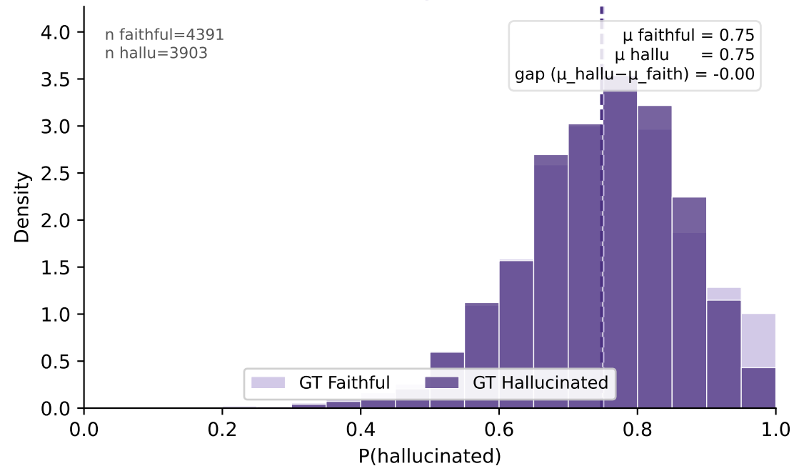
CheXagent-8B
