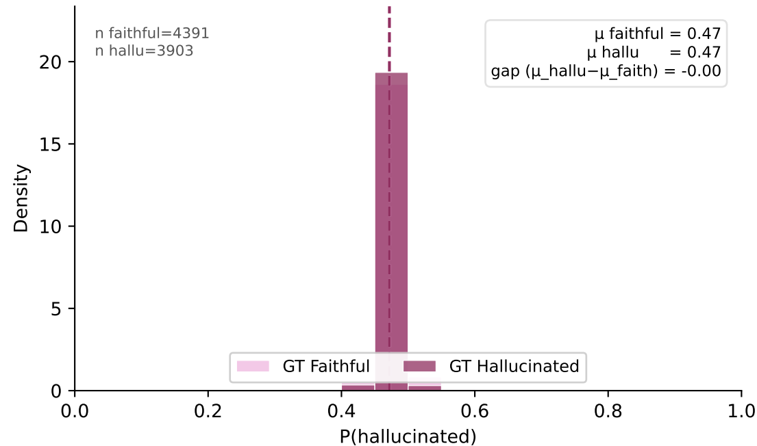
BiomedCLIP-300M
