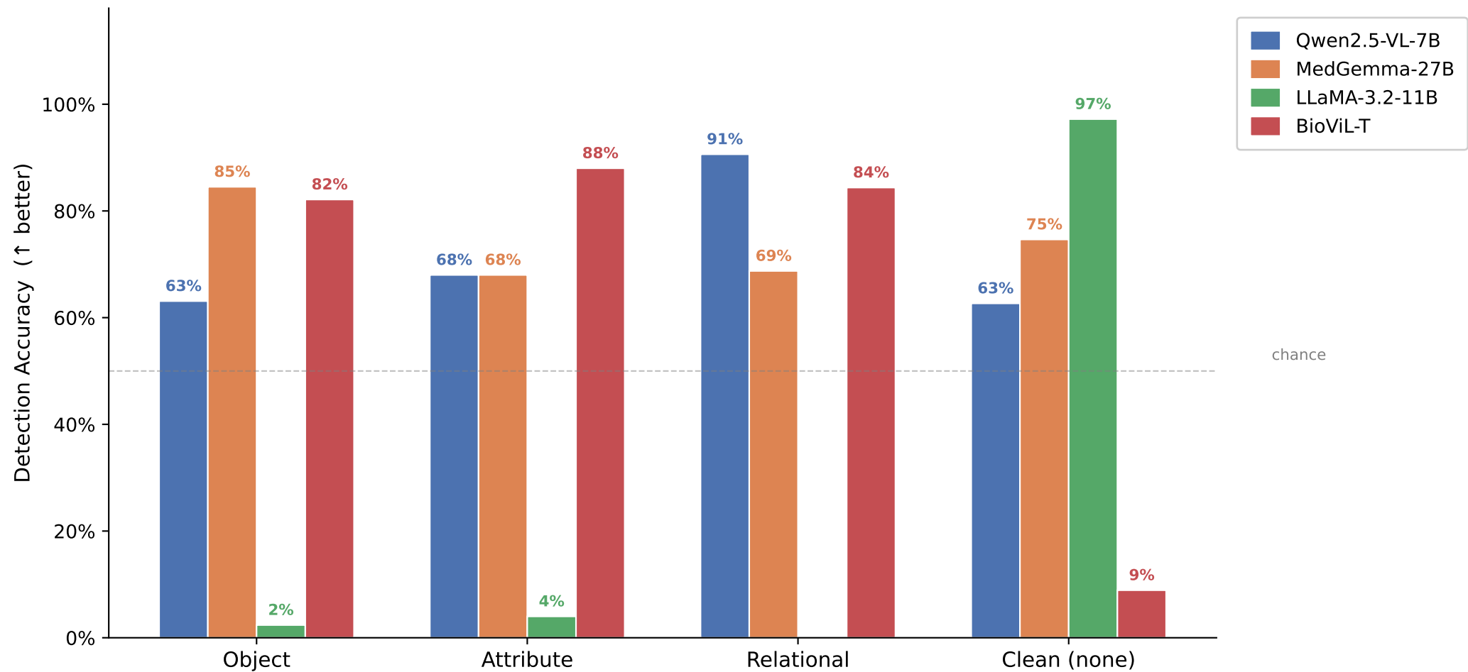
Per-Type Hallucination Detection Accuracy
