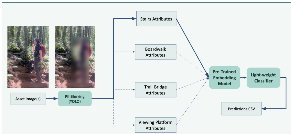
Figure 17: Final Data Pipeline Structure
