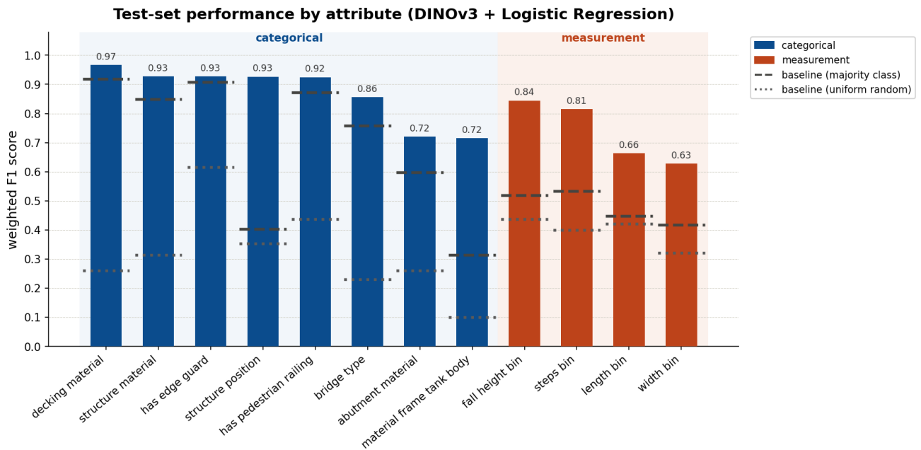
Figure 16: Weighted f1 scores of DINOv3 model on all 12 attributes, evaluated on a half-out test set
