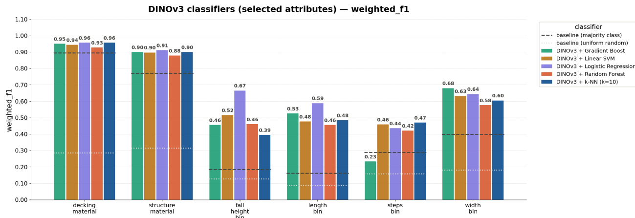
Figure 10: Dinov3 Embedding Model: Comparison across different classifier models
