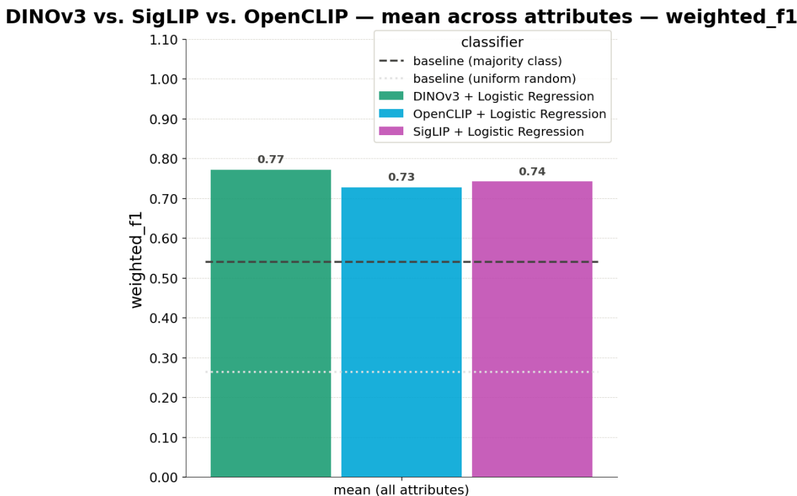
Figure 11: Dinov3 vs OpenClip vs Siglip: Comparison across different embedding models with logistic regression classifier (aggregated f1 across all 12 attributes)
