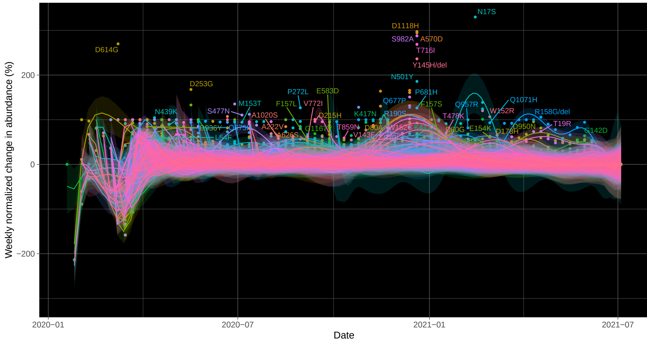
Emergence of SARS-CoV-2 spike protein variants
