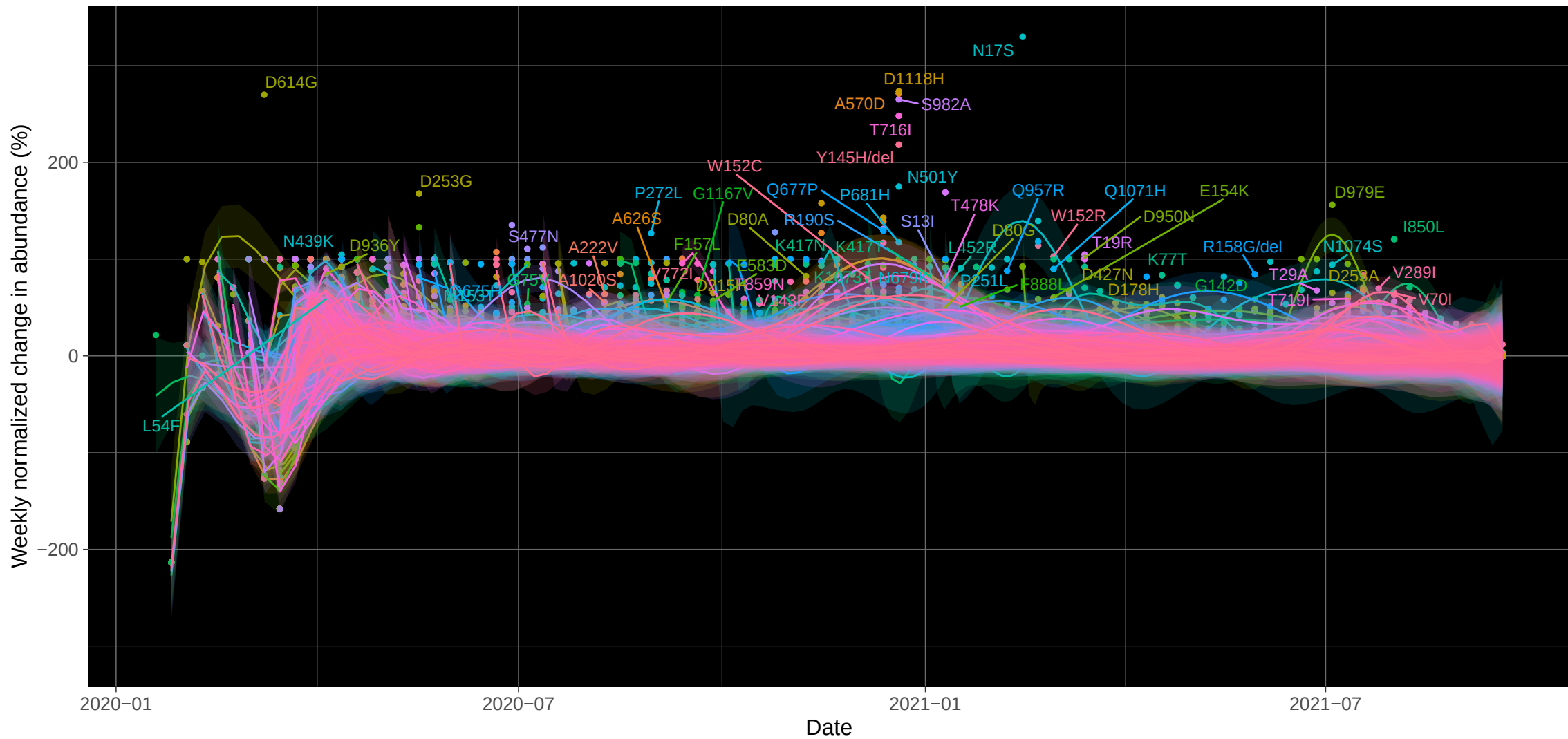
Emergence of SARS-CoV-2 spike protein variants
