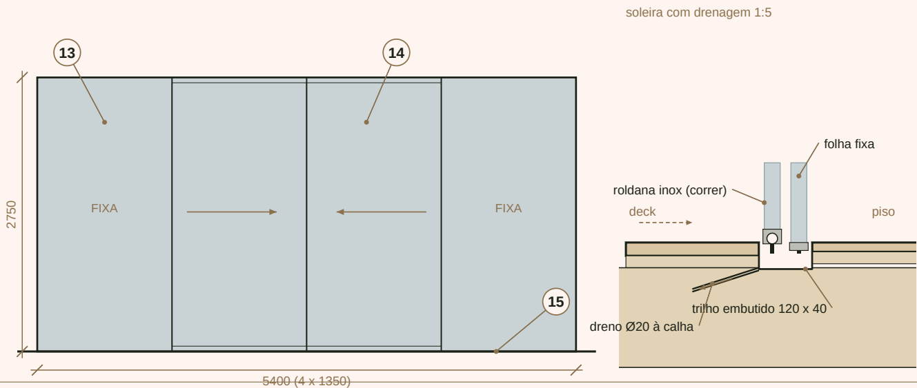
(C) FACHADA FRONTAL SAFARI 5400 X 2750: 2 FIXAS + 2 DE CORRER
