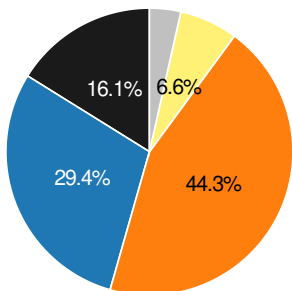
ACBI1-dependent (n=2,161)
