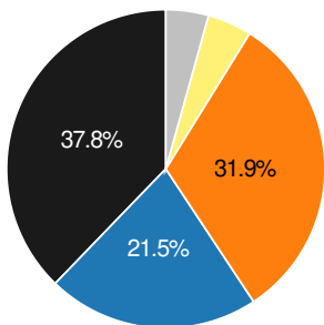
ACBI1-independent (n=21,560)
