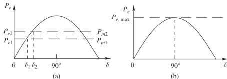
FIGURE 9.12 Steady state stability limit.
