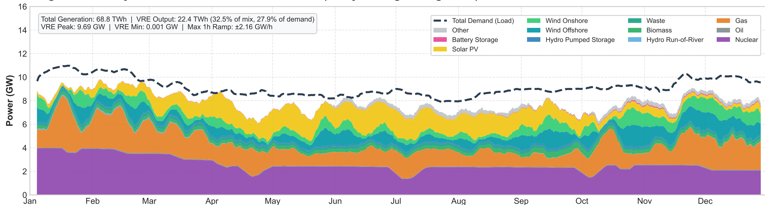
Belgian Electricity Generation Mix & Demand in 2025 (7-Day Rolling Average, GW)
