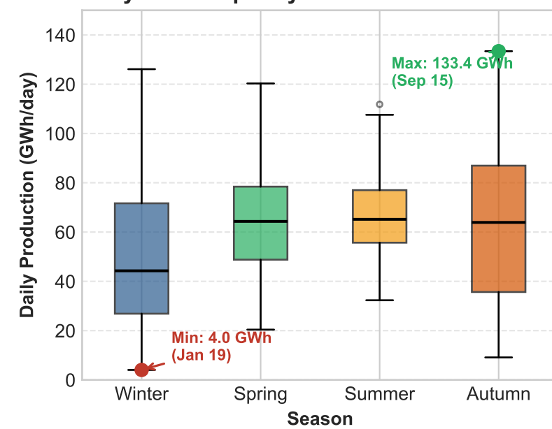
Daily VRE Output by Season
