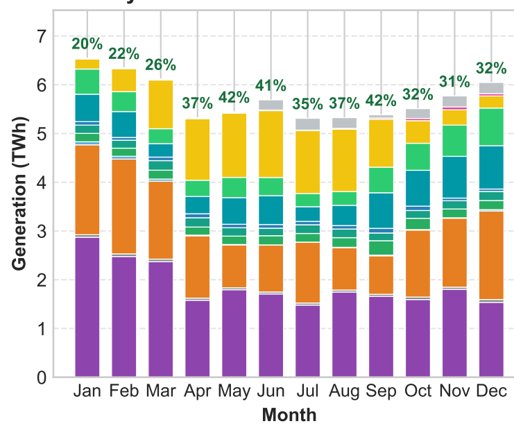
Monthly Generation Mix & VRE Share
