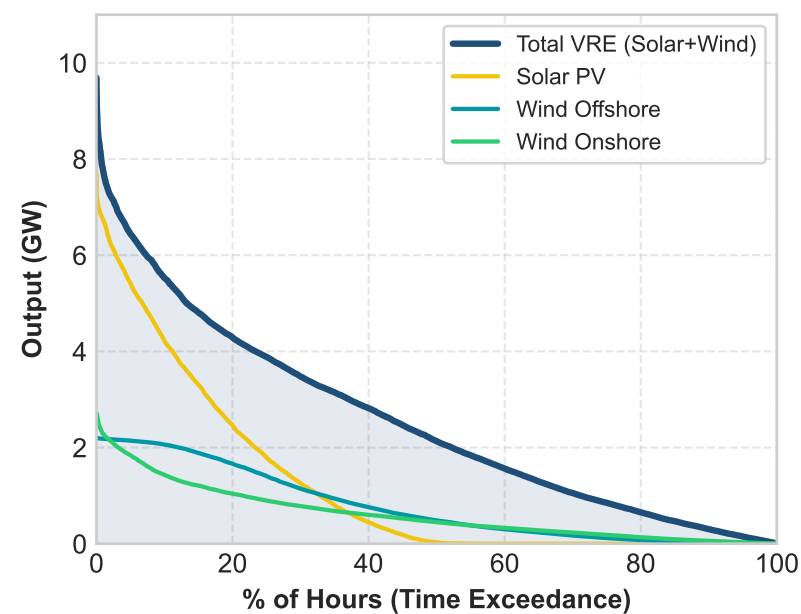
Renewable Duration Curves
