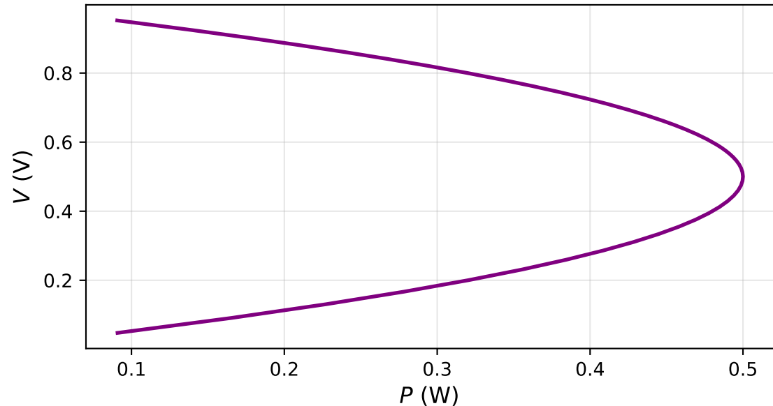
Voltage vs Power Transferred: E = 1 \text{ V} , R = 0.5 \text{ } \Omega
