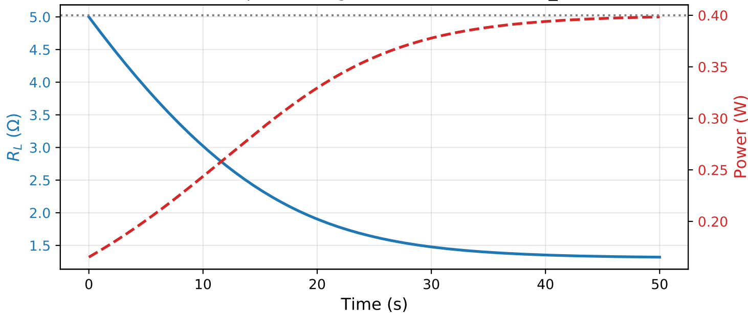
Controller response: target P_0 = 0.4 \text{ W} , initial R_L = 5 \Omega
