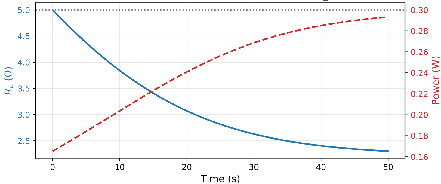
Controller response: target P_0 = 0.3 \text{ W} , initial R_L = 5 \Omega
