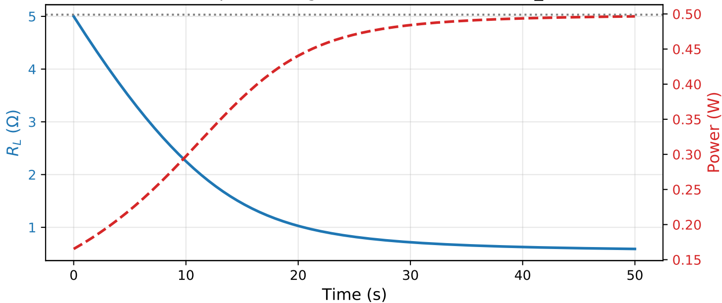
Controller response: target P0 = 0.499 W, initial R_L = 5 \Omega
