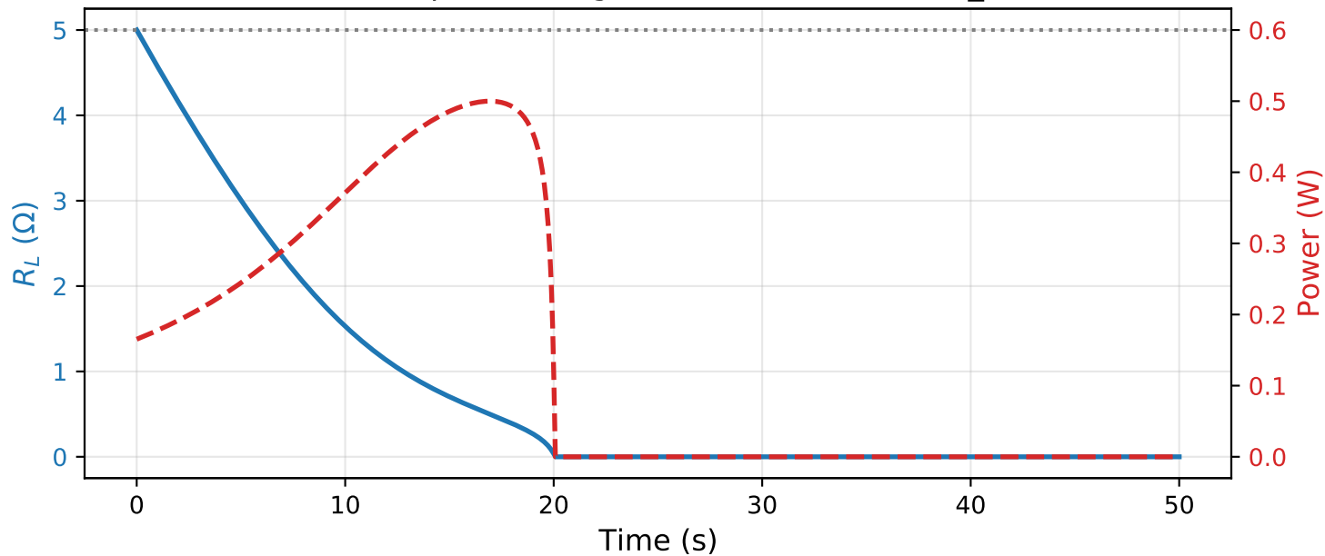
Controller response: target P_0 = 0.6 \text{ W} , initial R_L = 5 \Omega
