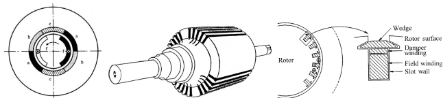
Cross-section of a round-rotor machine
