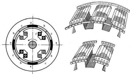
Cross-section of a salient-pole machine
