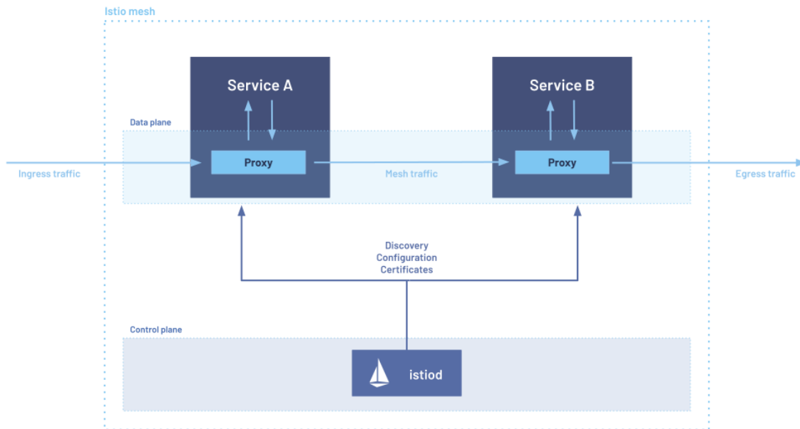
Figure 11.2: Istio Service Mesh
