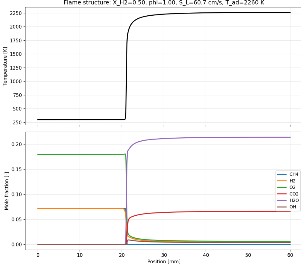
Figure 8: Flame structure (temperature and major species mole fractions) for the stoichiometric X_{H_2} = 0.5 flame.
