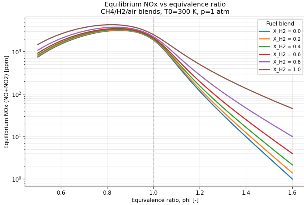
Figure 2: Equilibrium \text{NO}_x ( \text{NO} + \text{NO}_2 ) vs equivalence ratio for \text{CH}_4/\text{H}_2/\text{air} blends.
