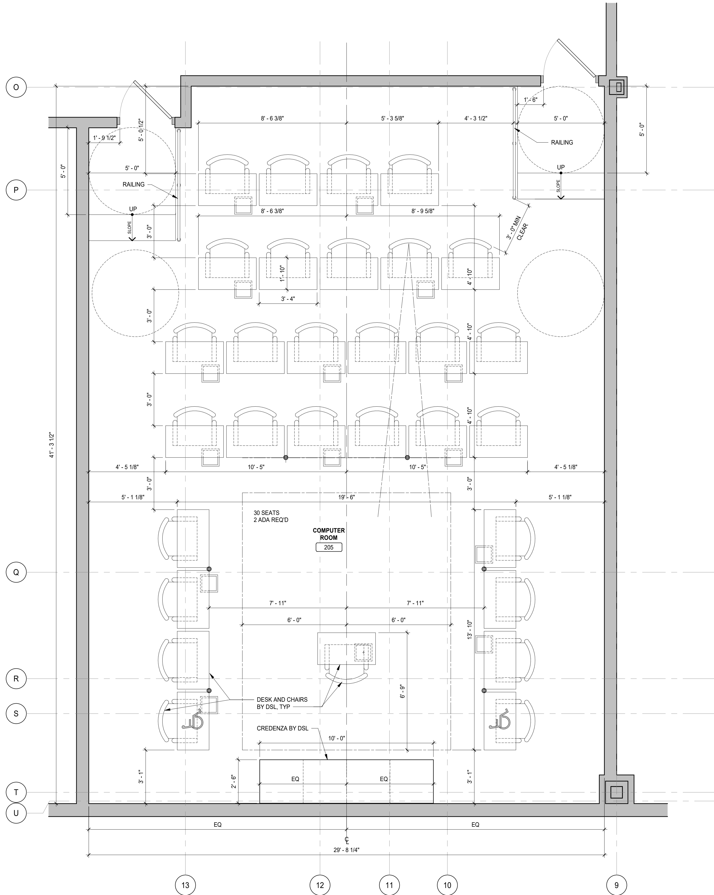
2 SECOND FLOOR FURNITURE PLAN - OPTION 2 3/8" = 1'-0"
