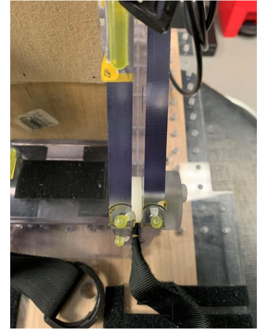
Axis assembly/rotary joint for foot pedal (Note fiducial markers for alignment to biomechanical calculations)
