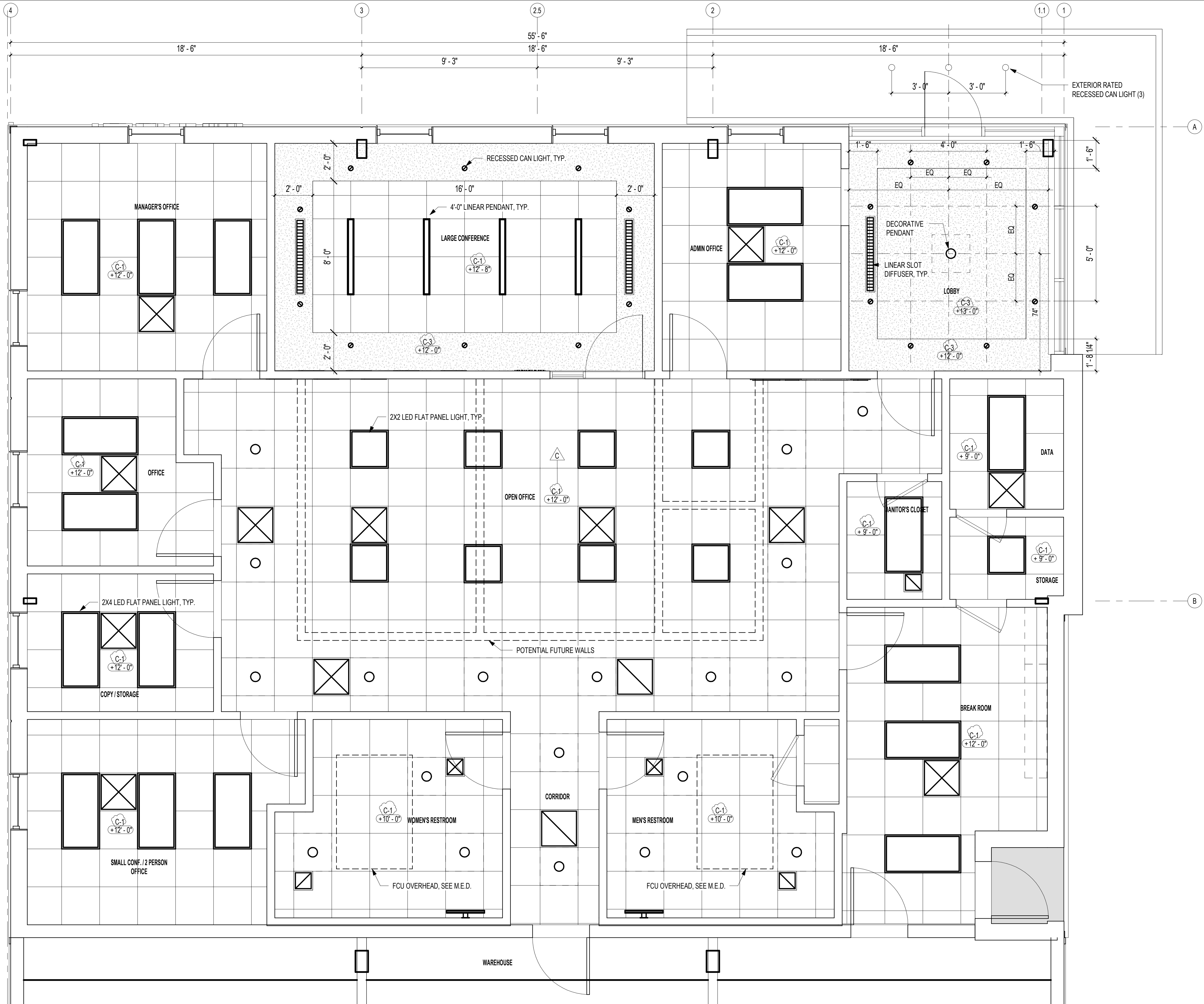
REFLECTED CEILING PLAN 1 3/8" = 1'-0"
