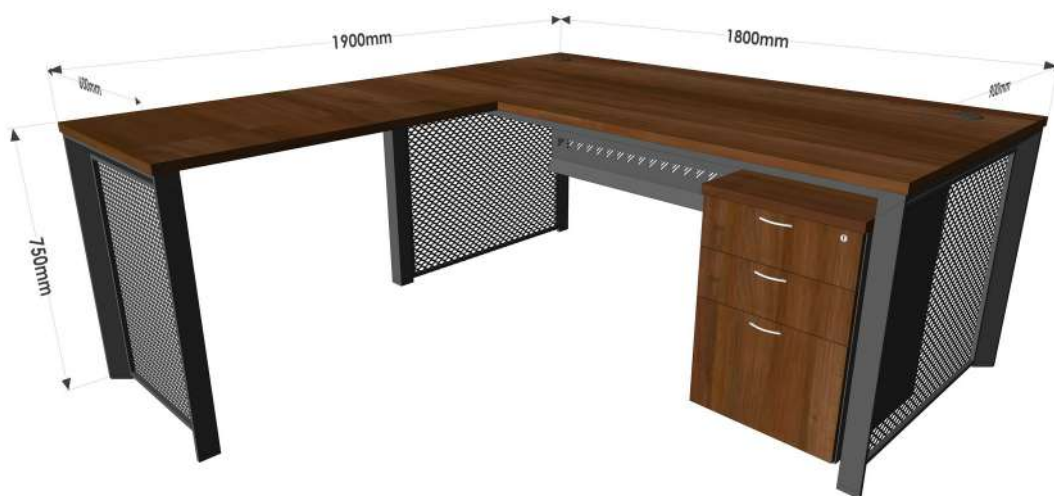
ST-MS01 Director Table 1800W x 1900D x 750H mm
