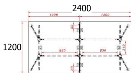
ST-SQAMT 2400 Meeting Table 2400W x 1200D x 750H mm
