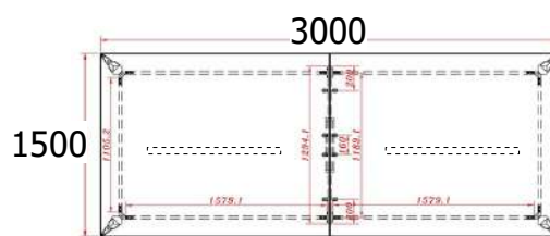
ST-YOUNG 3000 Workstation Table 3000W x 1500D x 750H mm
