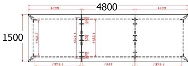
ST-YOUNG 4800 Workstation Table 4800W x 1500D x 750H mm
