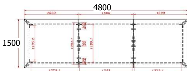
ST-YOUNGMT 4800 Meeting Table 4800W x 1500D x 750H mm
