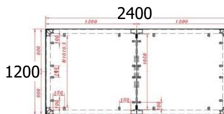
ST-TRIMT 2400 Meeting Table 2400W x 1200D x 750H mm
