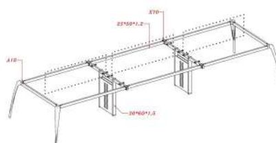
ST-YOUNG 3000 Workstation Table 3000W x 1500D x 750H mm
