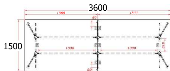
ST-SQAMT 3600 Meeting Table 3600W x 1500D x 750H mm
