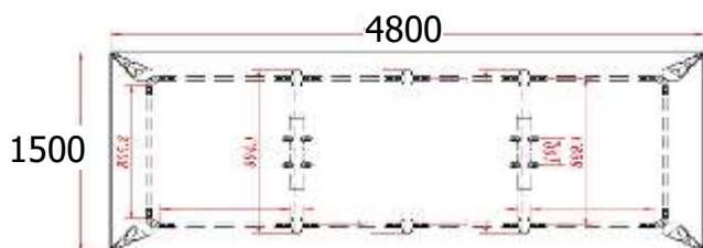
ST-Delta MT 4800 Meeting Table 4800W x 1500D x 750H mm
