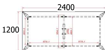
ST-Delta MT 2400 Meeting Table 2400W x 1200D x 750H mm
