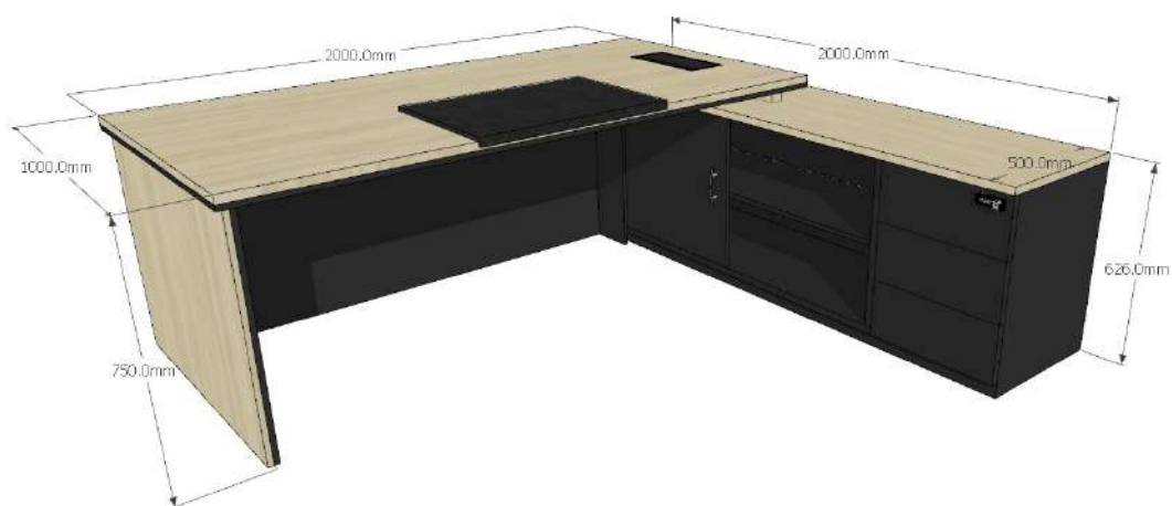
ST-MN01 Director Table 2000W x 1000D x 750H mm
