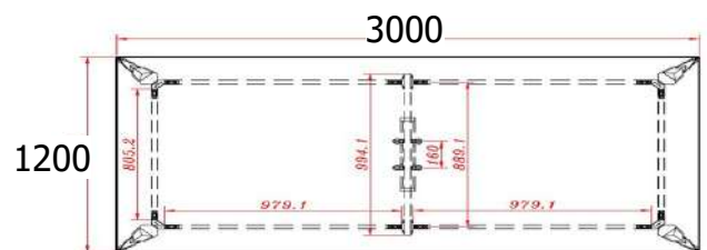
ST-Delta Work 01 Workstation Table 3000W x 1200D x 750H mm
