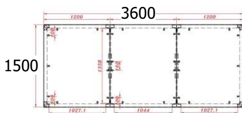
ST-TRIMT 3600 Meeting Table 3600W x 1500D x 750H mm
