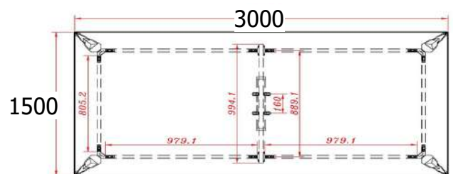
ST-Delta Work 02 Workstation Table 3000W x 1500D x 750H mm
