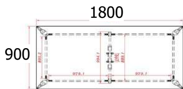
ST-Delta MT 1800 Meeting Table 1800W x 900D x 750H mm
