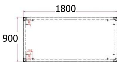
ST-TRIMT 1800 Meeting Table 1800W x 900D x 750H mm
