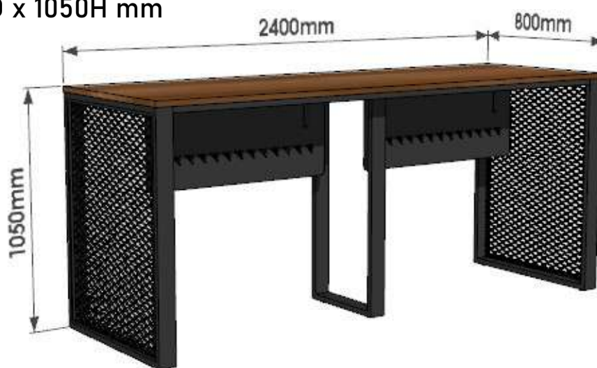
MS50 2400W x 800D x 1050H mm
