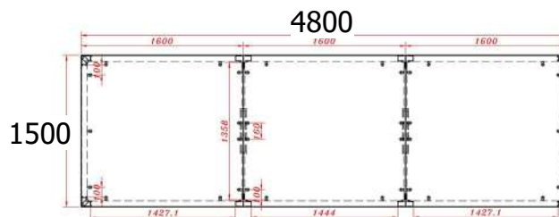
ST-TRIMT 4800 Meeting Table 4800W x 1500D x 750H mm
