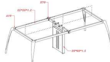
ST-YOUNG 3000 Workstation Table 3000W x 1500D x 750H mm
