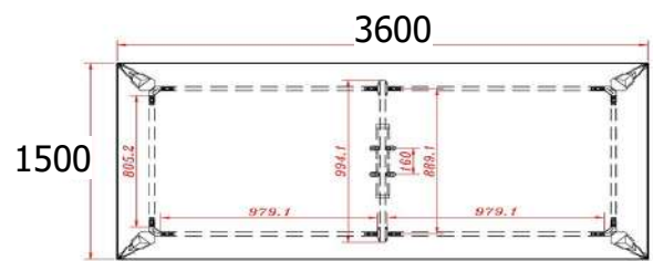
ST-Delta MT 3600 Meeting Table 3600W x 1500D x 750H mm
