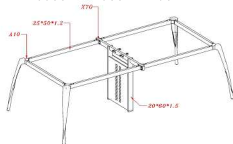
ST-YOUNGMT 3600 Meeting Table 3600W x 1500D x 750H mm
