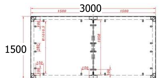
ST-TRIMT 3000 Meeting Table 3000W x 1500D x 750H mm
