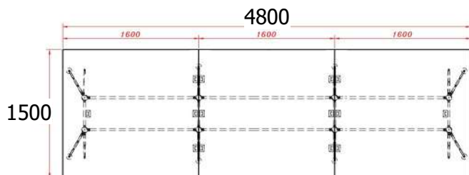
ST-SQAMT 4800 Meeting Table 4800W x 1500D x 750H mm
