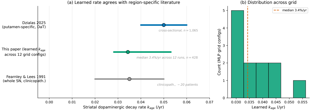
Fig. 5: Learned striatal age-decay rate versus published estimates. (a) Horizontal range plots for Fearnley & Lees 1991 6 (whole substantia nigra, clinicopathological), this paper’s learned k_{age} across the twelve MLP-grid configurations, and Dzialis 2025 3 (putamen-specific, DaT-SPECT longitudinal). Dots mark median values; bars span published or measured ranges. (b) Histogram of learned k_{age} across the twelve grid configs with the median indicated.
