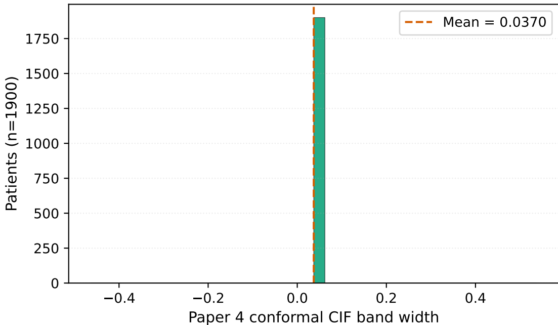
Fig. 3. Per-patient conformal CIF band widths (IPCW, 90% CL) from Paper 4.
