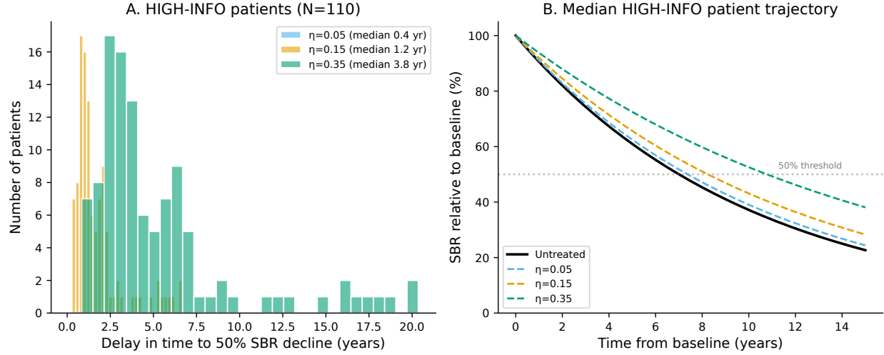
Figure 9.5: Prasinezumab counterfactual simulation. (A) Delay distribution across scenarios for HIGH-INFO patients. (B) Median trajectory under treatment.
