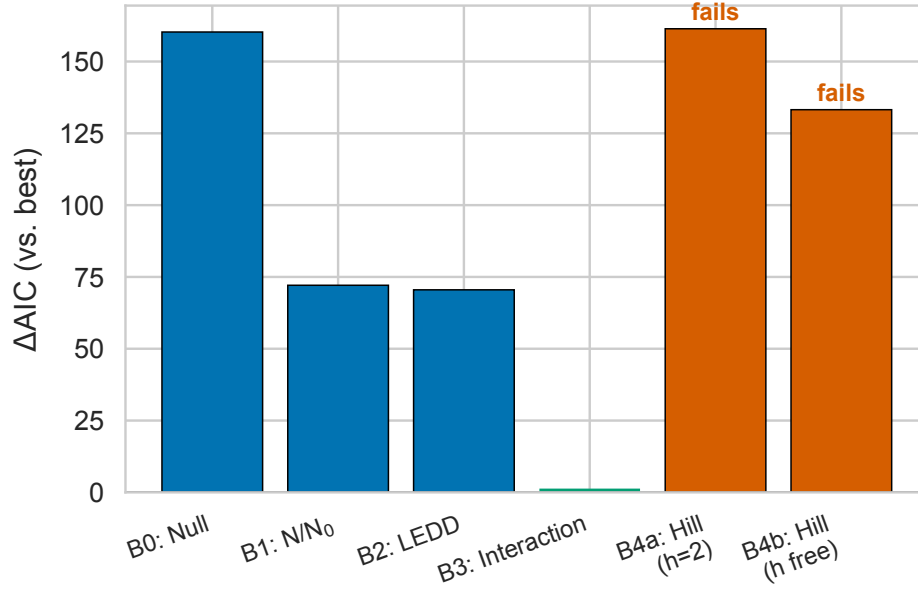
Figure 12.6: Path B: \Delta AIC relative to the interaction model (B3). Positive values indicate worse fit. The interaction model decisively outperforms all alternatives ( |\Delta AIC| > 10 ; Burnham & Anderson threshold). The Hill models (B4a, B4b) perform worse than the null model, confirming the sub- EC_{50} regime.
