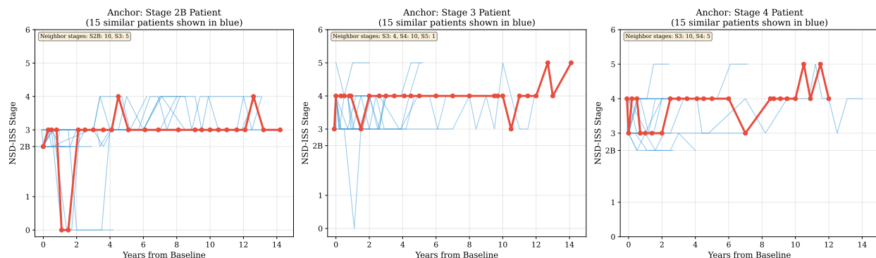
Figure 5.4: “Patients like you” trajectory analysis. For three anchor patients (one per clinical stage: 2B, 3, 4), the red bold line shows the anchor patient’s actual NSD-ISS trajectory over time. Blue lines show trajectories of the 15 most similar patients identified by the graph. Graph-DT uses these population-level trajectory patterns to enrich individual predictions—for example, a stage 2B patient’s neighbors are predominantly stage 3, providing direct evidence about likely progression timing.
