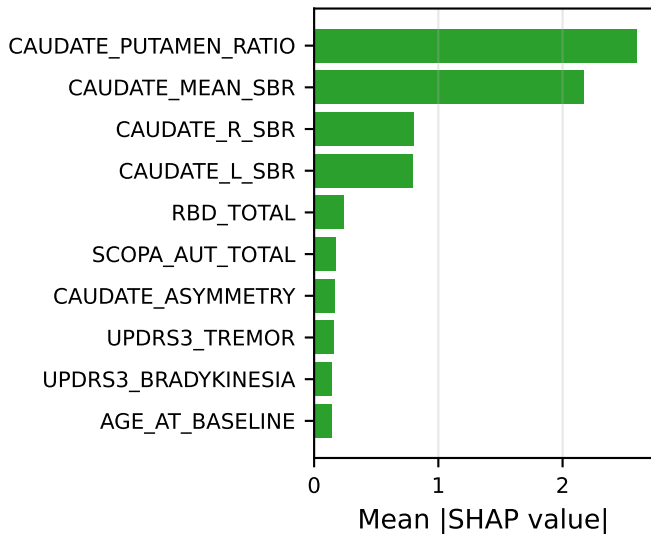
(a) Top-10 SHAP features — CatBoost binary
