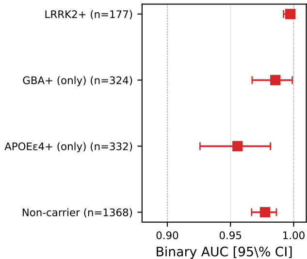
(b) Subgroup fairness by genetic carrier status
