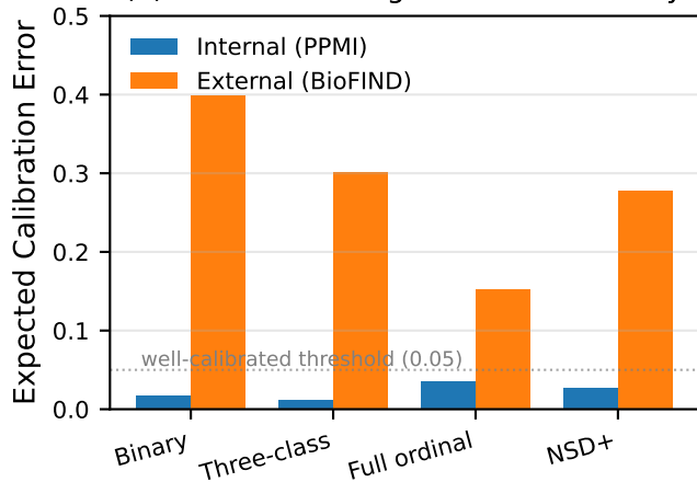
(a) ECE — 10× degradation externally
