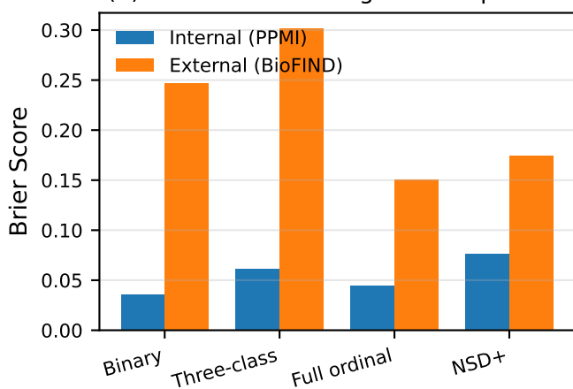
(b) Brier — similar degradation pattern
