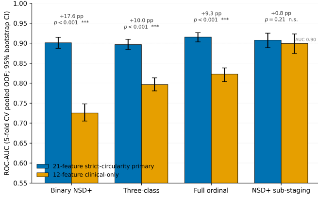
Fig. 4. Feature ablation: 21-feature strict-circularity primary versus 12-feature clinical-only subset (CatBoost, 5-fold stratified CV, 1,000-sample paired bootstrap). Removing imaging + genetics features is essential for binary NSD+ classification (paired \Delta = -0.176 , 95% CI [-0.200, -0.155] , p < 0.0001 ) but statistically indistinguishable for NSD+ sub-staging ( \Delta = +0.008 , 95% CI [-0.005, +0.022] , p = 0.21 ). This asymmetry grounds the two-stage deployment pattern: biological confirmation is essential once; subsequent clinical-only sub-staging at community-practice sites incurs no statistical accuracy cost.
