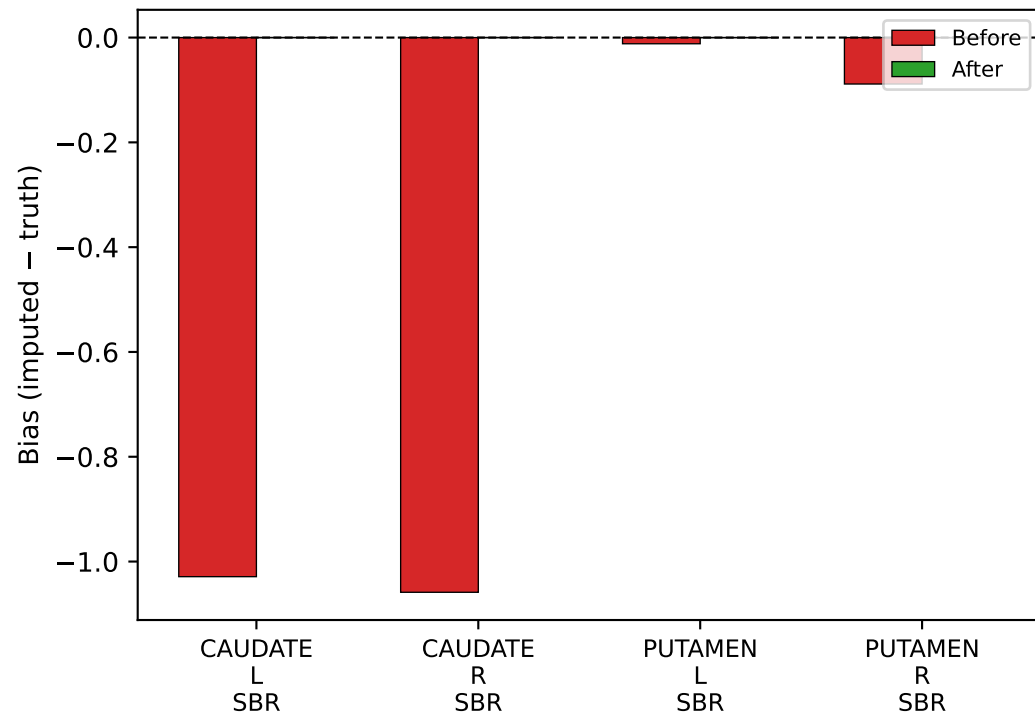
(b) Bias before vs after bias correction
