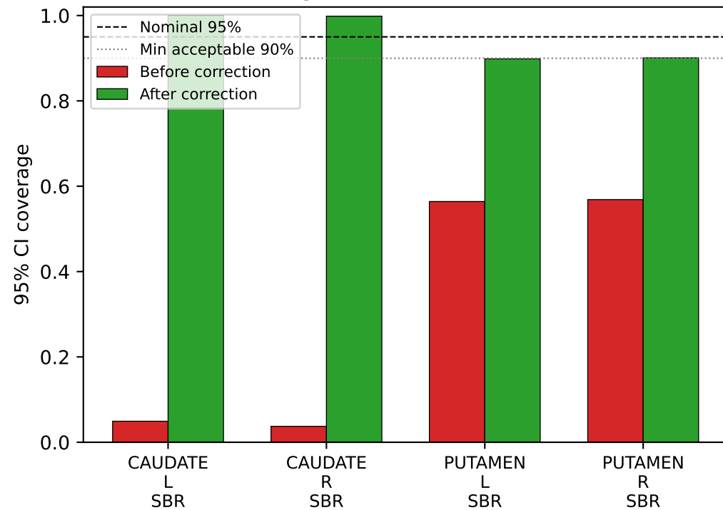
(a) Coverage before vs after calibration
